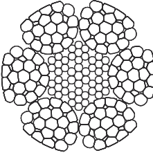
6x25 (12/6/6/1) POWER PAC
